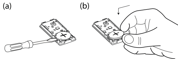
Figure 9: Battery removal and insertion
