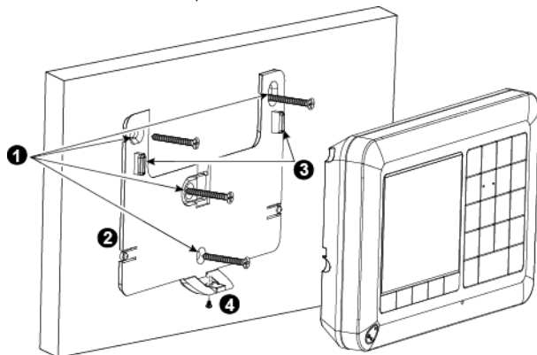
Figure 3 : montage mural
