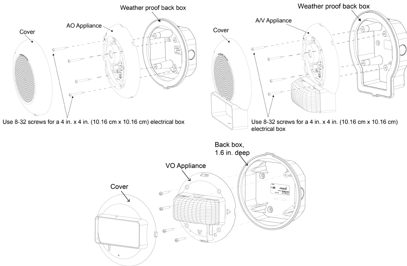
Figure 2: Installation reference
