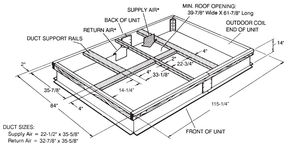
Figure 8: ZF180 Roof Curb
