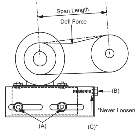
Figure 18: Belt Adjustment
