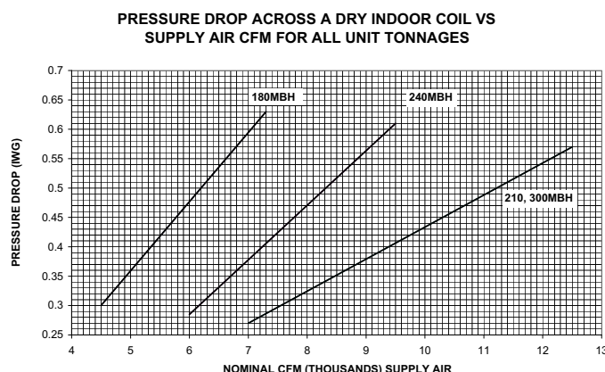
Figure 20: Pressure Drop Across A Dry Indoor Coil Vs. Supply Air CFM For All Unit Tonnages
