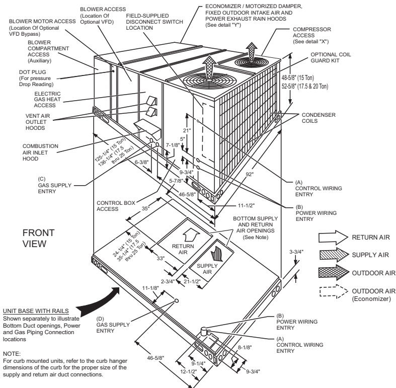
Figure 5: ZF180-300 Unit Dimensions Front View
