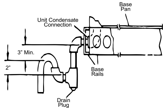
Figure 11: Condensate Drain
