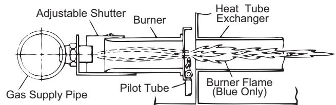
Figure 24: Typical Flame
