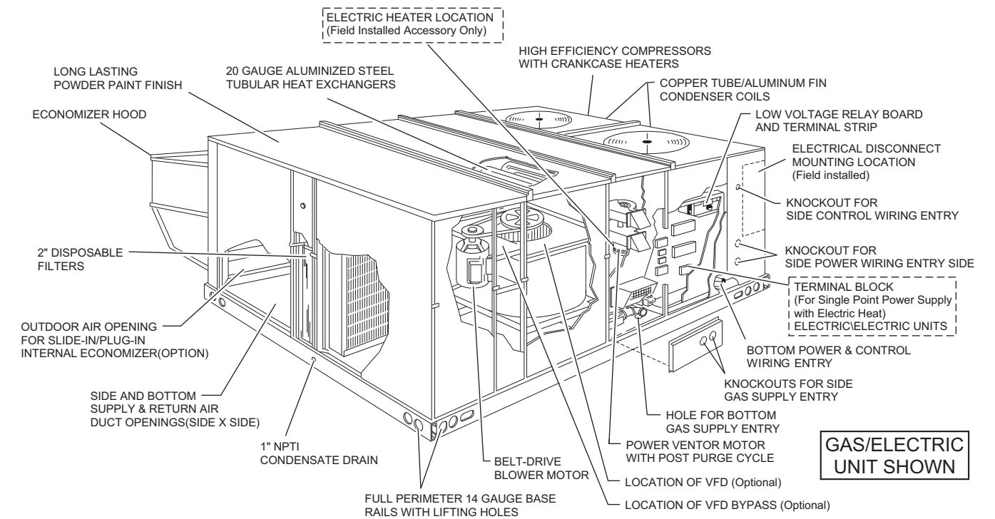
Figure 1: ZF180-300 Component Location
