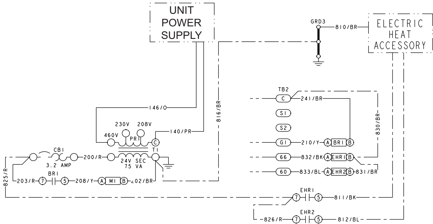
Figure 9: Typical Field Wiring Diagram – NC090 Evaporator
