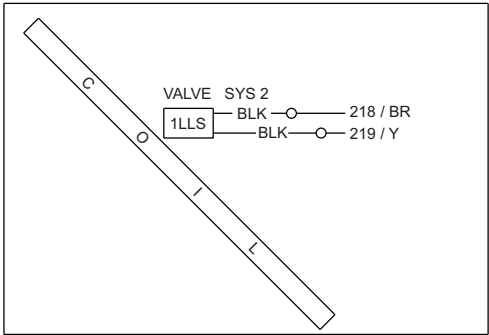
Figure 11: Typical NC120 - 240 Liquid Line Solenoid Wiring
