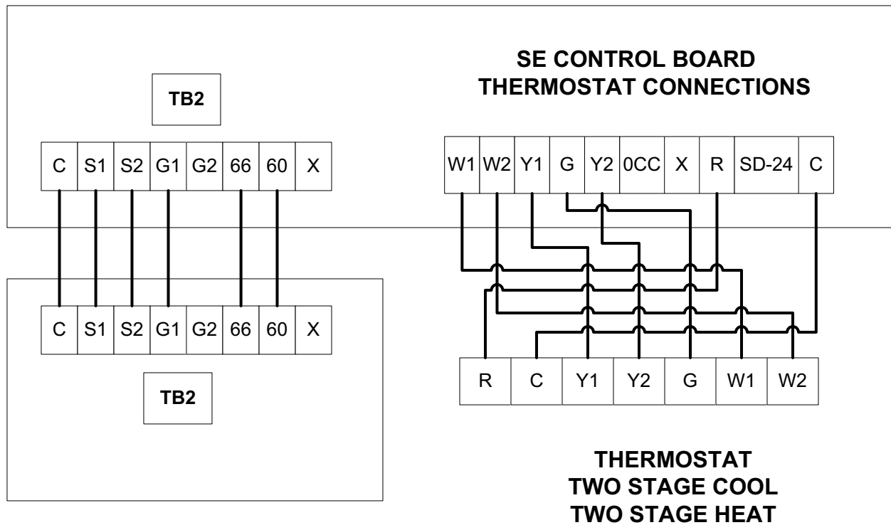
Figure 17: Typical field 24 volt control wiring diagram – NC120 thru 240 Evaporator with YC120 thru 240 Condenser
