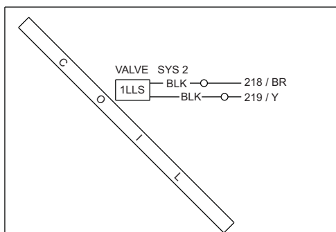
Figure 18: Typical NC120 - 240 Liquid Line Solenoid Wiring
