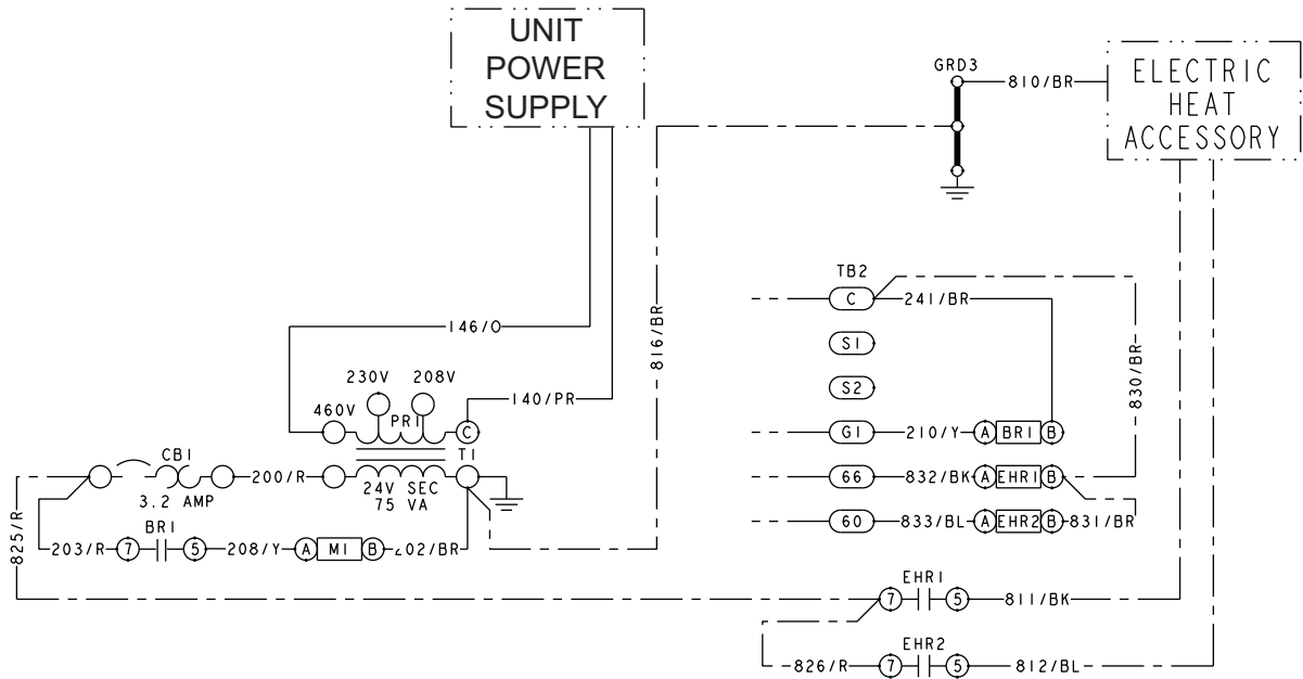
Figure 16: Typical Field Wiring Diagram – NC090 Evaporator
