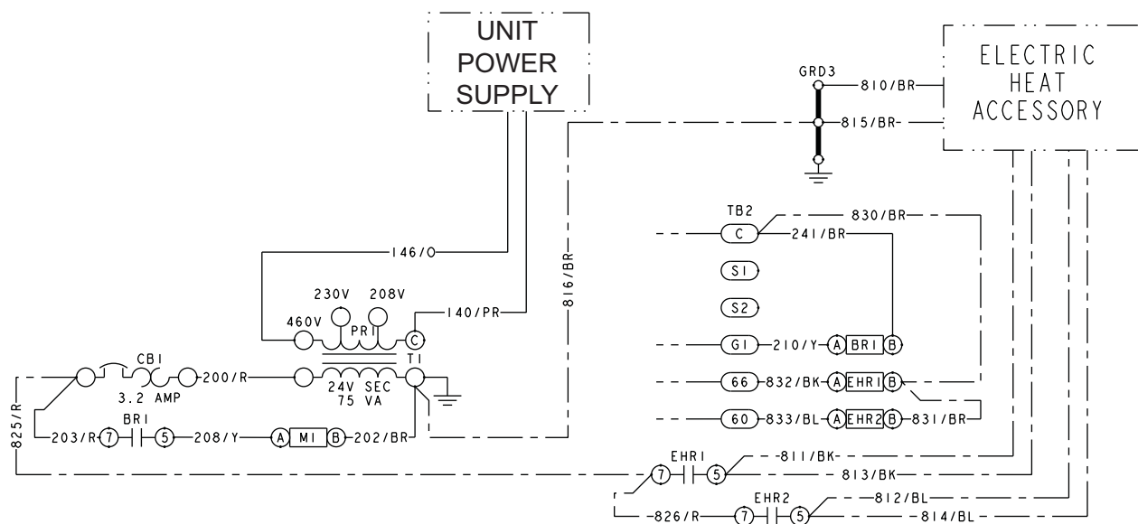
Figure 21: Typical Field Wiring Diagram – ND120 thru 240 Evaporator
