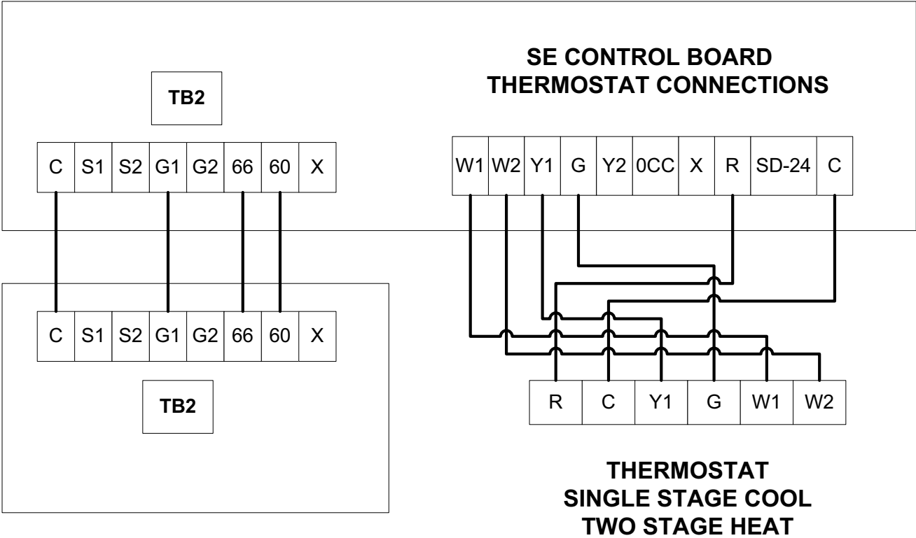
Figure 15: Typical field 24 volt control wiring diagram – NC090 Evaporator with YC090 Condenser
