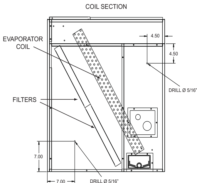
Figure 23: Hole Location For Pressure Drop Reading
