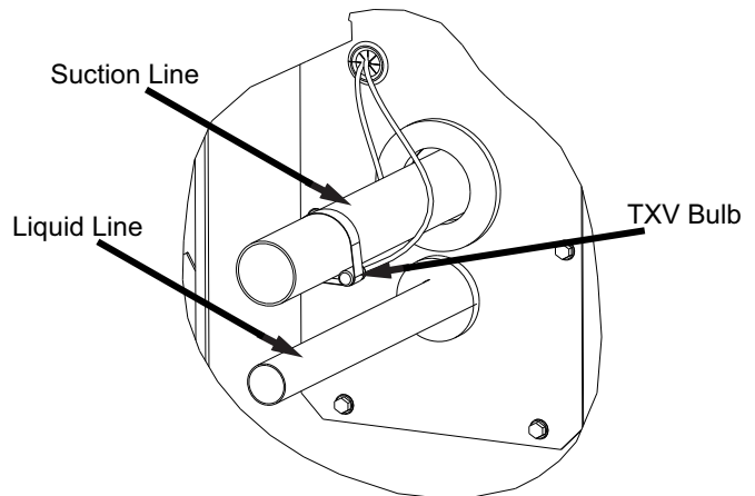
Figure 7: TXV Bulb Location
