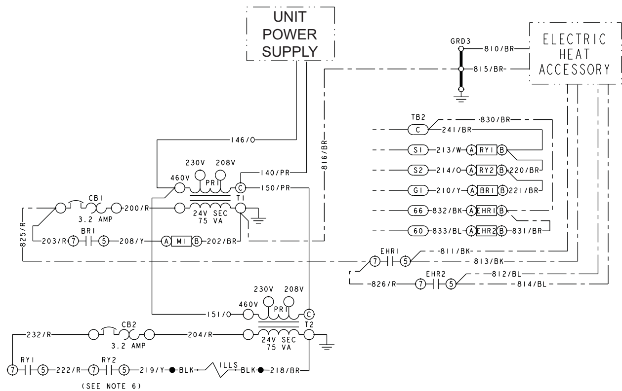
Figure 12: Typical Field Wiring Diagram – NC120 thru 180 Evaporator
