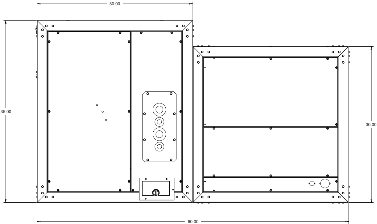
Figure 24: Unit Dimensions NC090/120 & ND120 (Continued)
