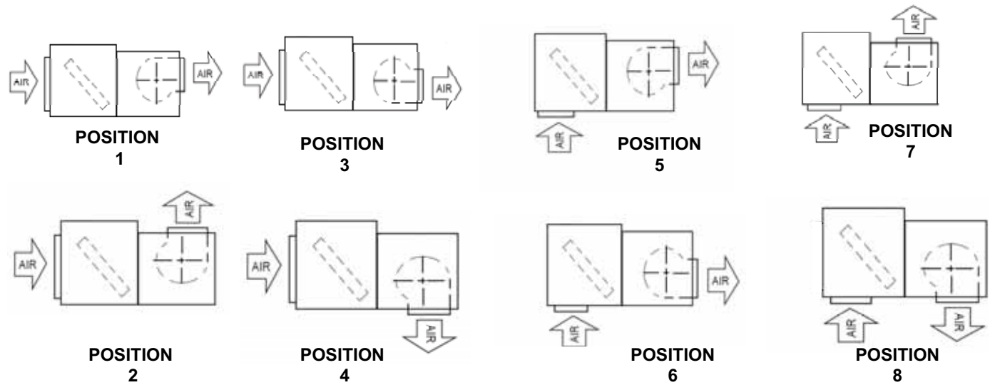
Figure 2: Horizontal Airflow Arrangements
