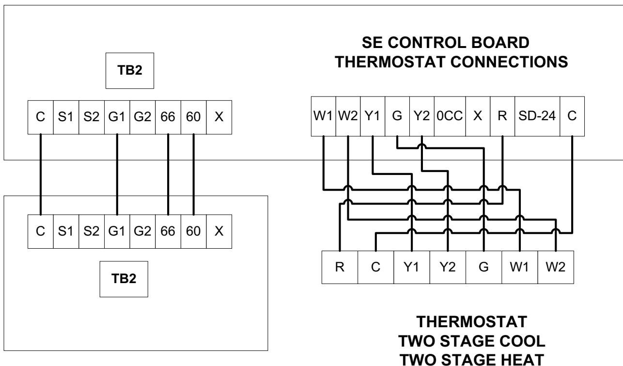
Figure 20: Typical field 24 volt control wiring diagram – ND120 thru 240 Evaporator with YD120 thru 240 Condenser
