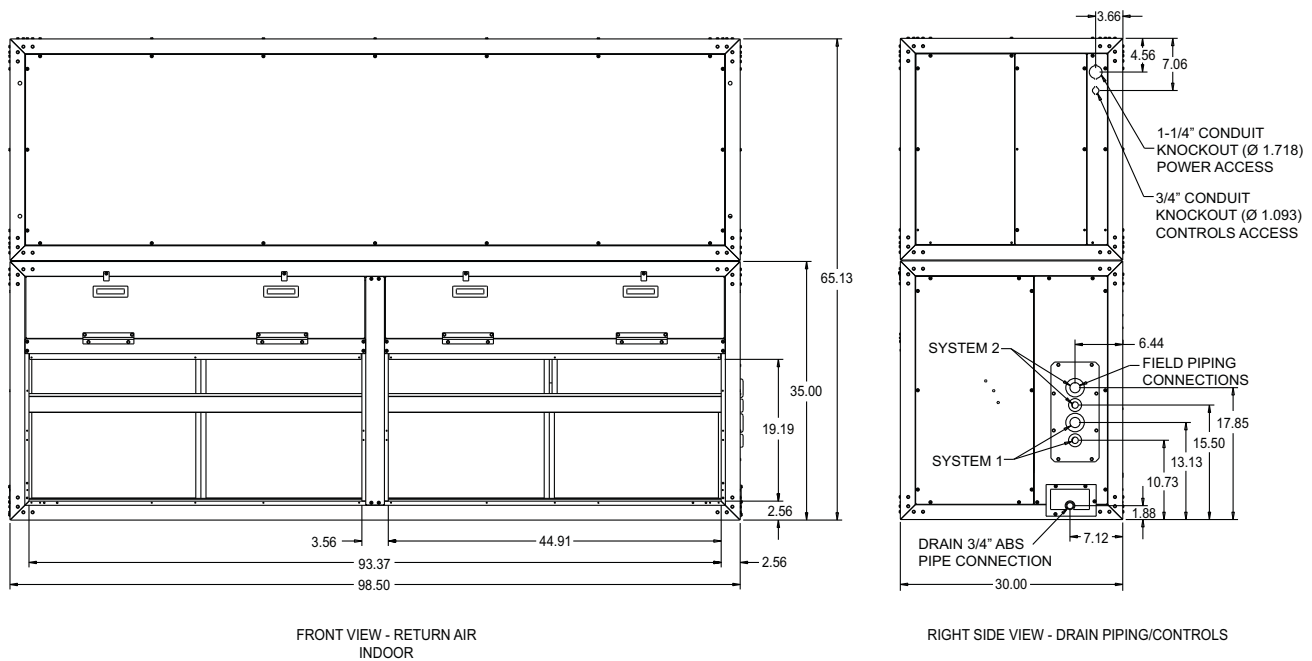
Figure 29: Unit Dimensions NC/ND240
