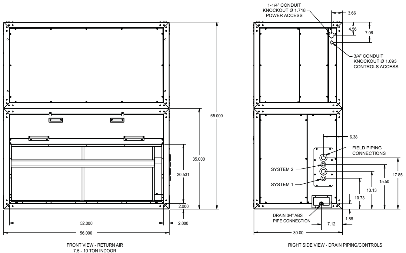
Figure 27: Unit Dimensions NC090/120 & ND120
