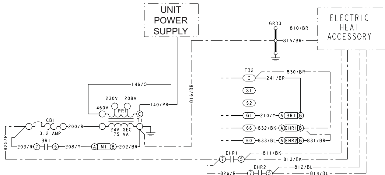
Figure 14: Typical Field Wiring Diagram – ND180 thru 240 Evaporator
