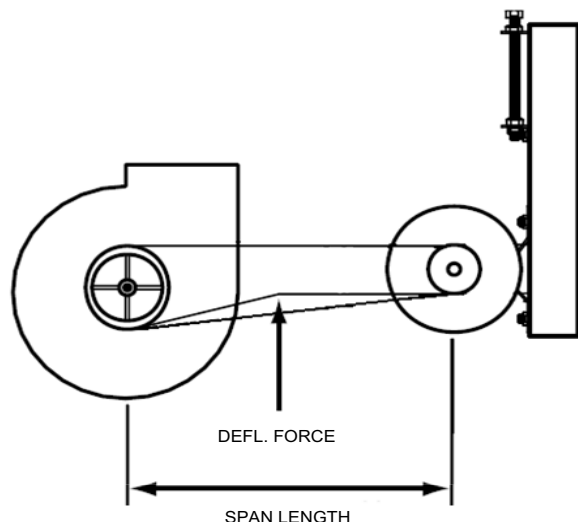
Figure 25: Belt Adjustment
