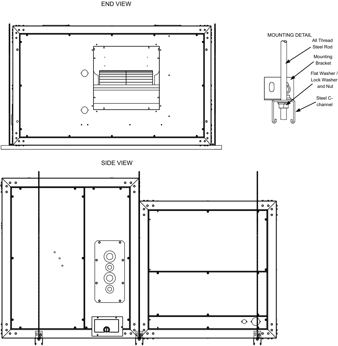
Figure 4: Typical Suspension of AHU's From Ceiling
