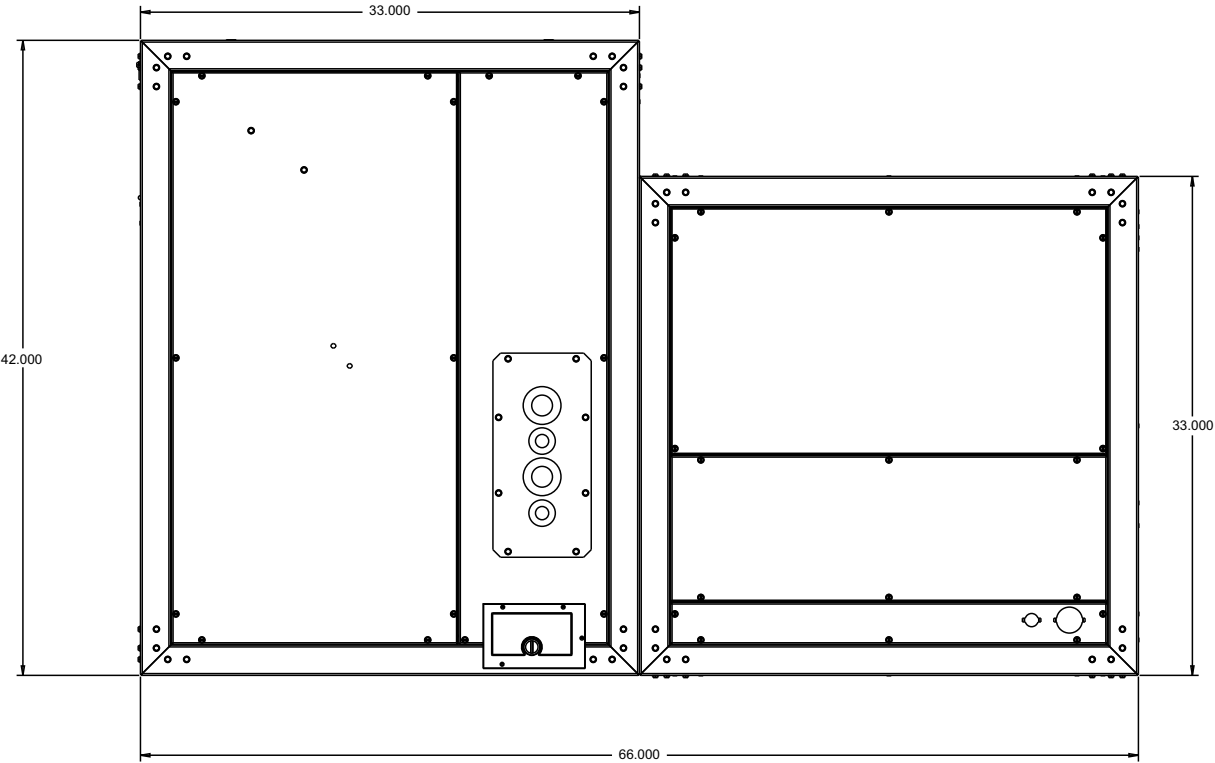
Figure 25: Unit Dimensions NC/ND180 (Continued)
