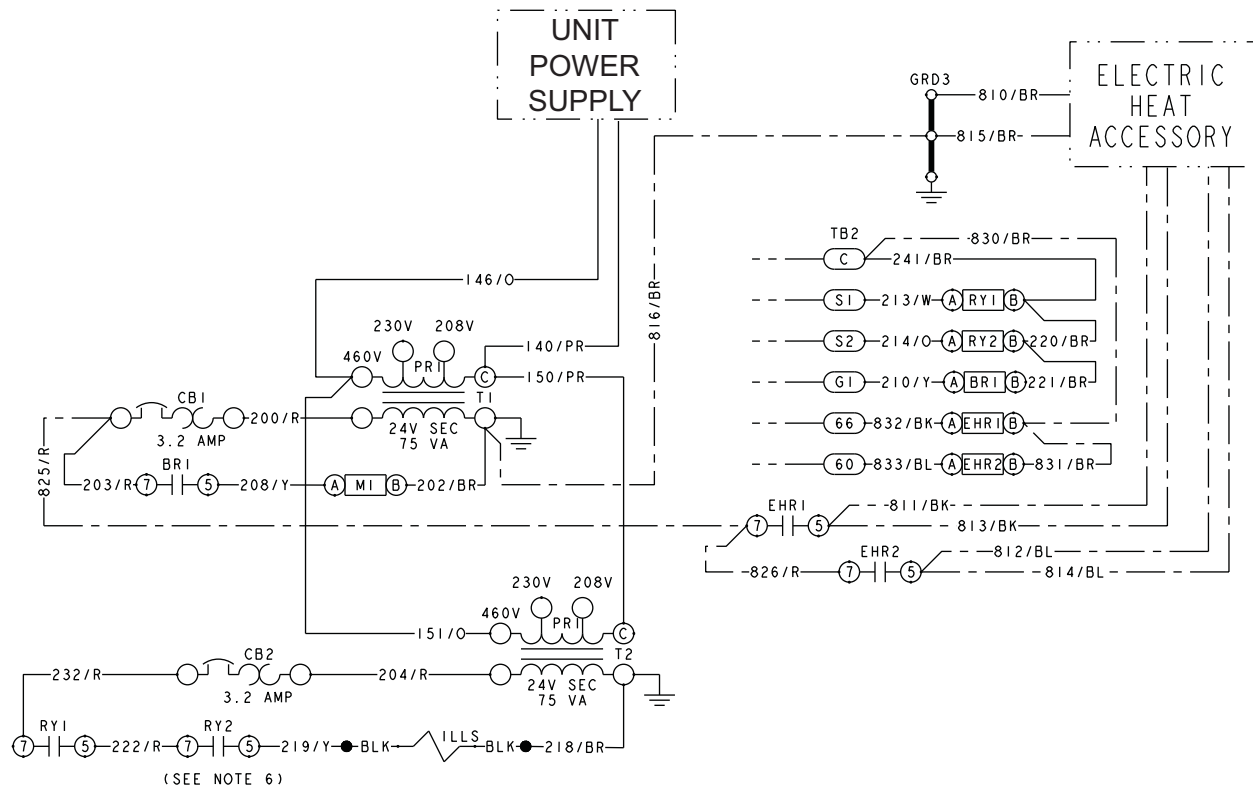
Figure 19: Typical Field Wiring Diagram – NC120 thru 240 Evaporator
