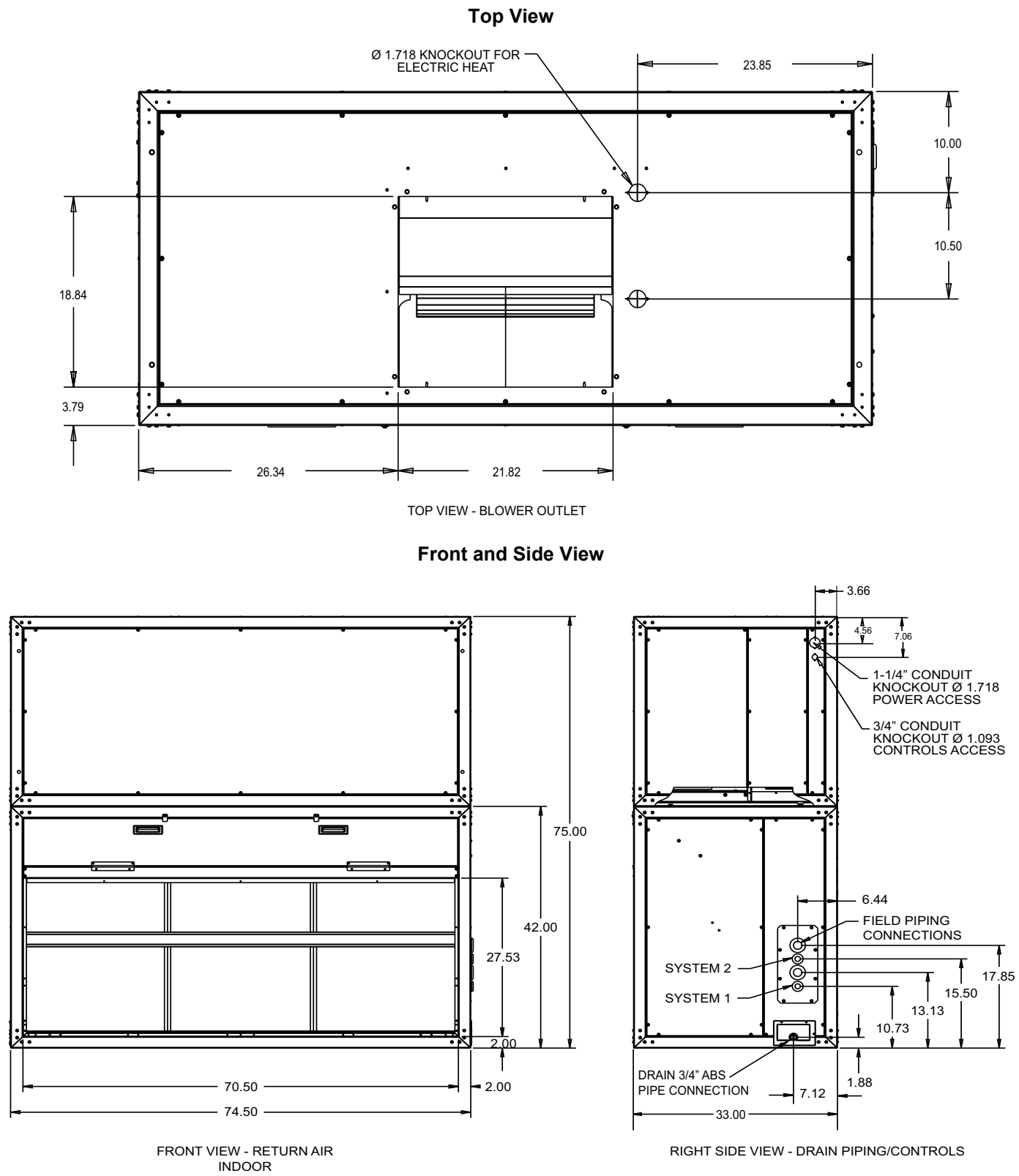
Figure 28: Unit Dimensions NC/ND180
