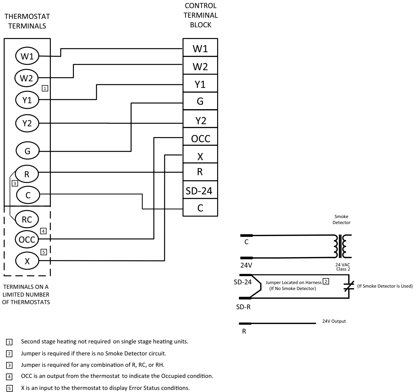
Figure 12: Typical Field Control Wiring
