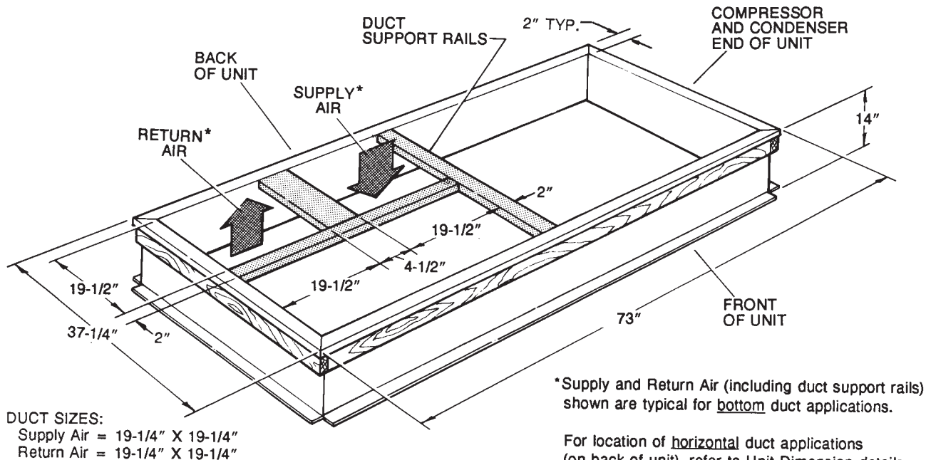
Figure 9: XN036-060 Roof Curb
