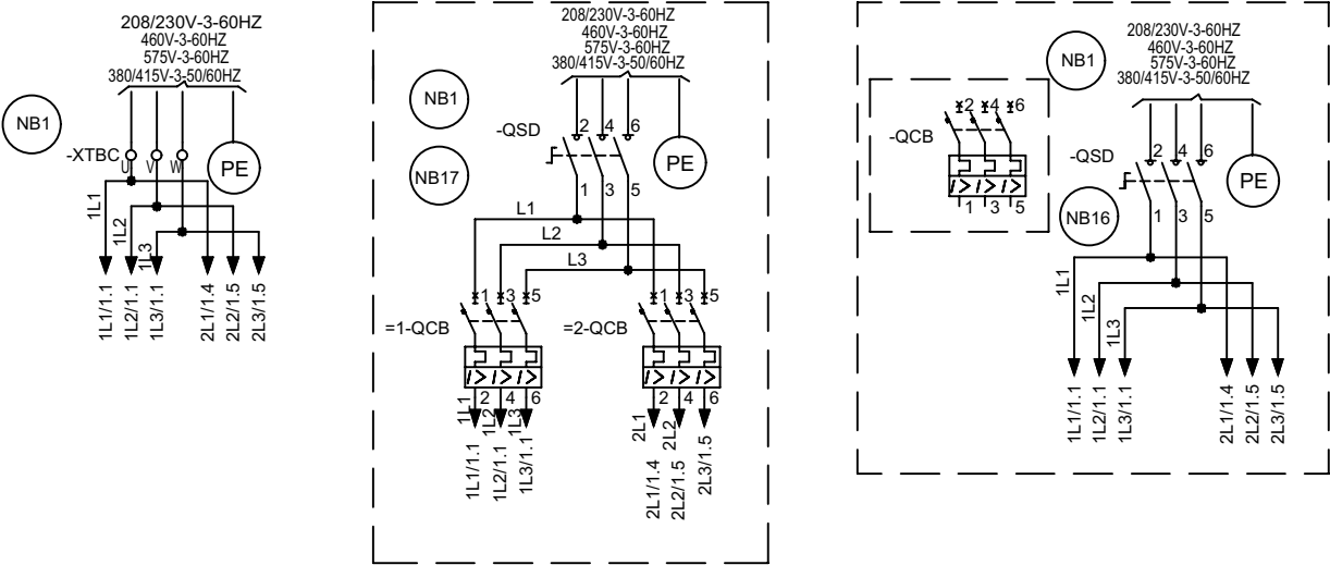
SINGLE POINT WIRING OPTIONS
