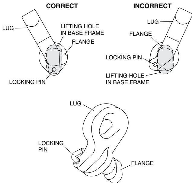
Figure 8: Lifting lugs
