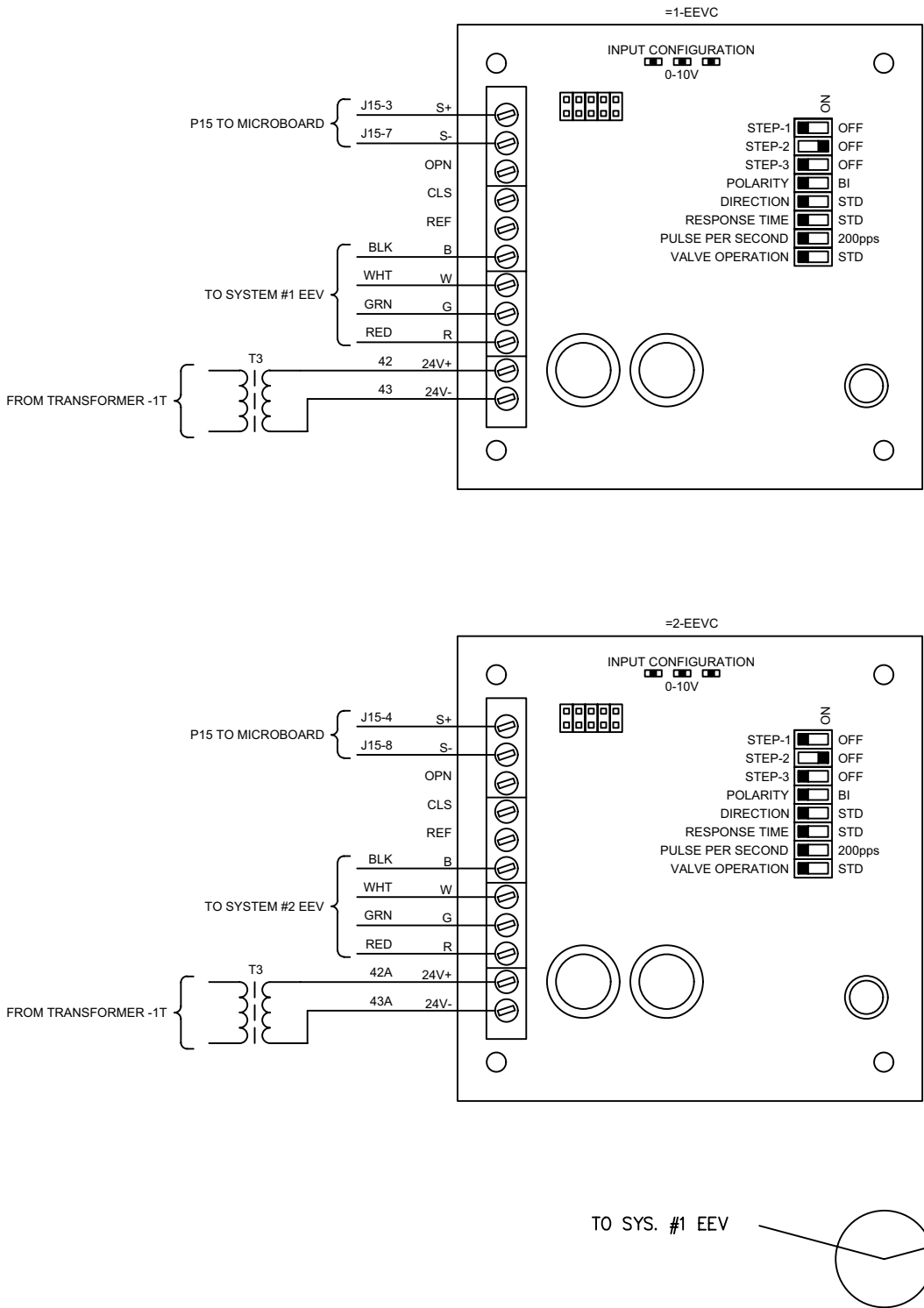
Figure 21: EEV Controller Elementary Diagram
