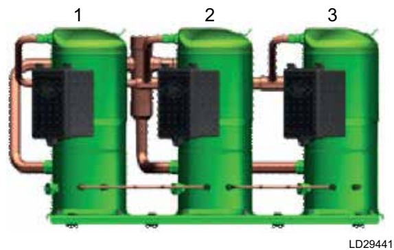
Figure 42: Trio Set
