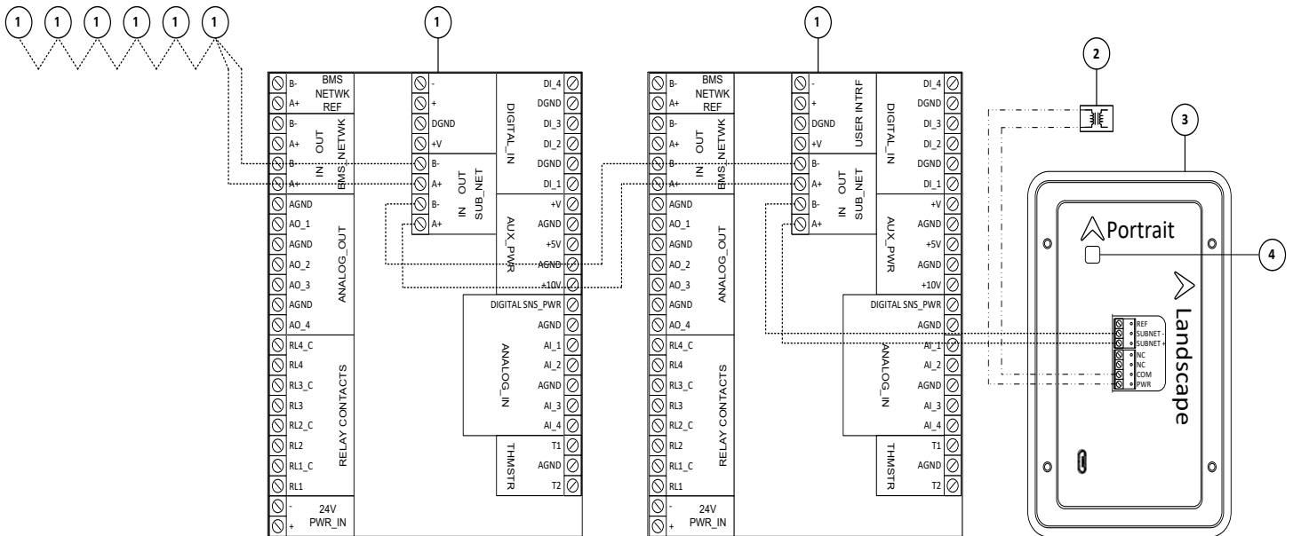
Figure 9: Daisy chain of FMS and/or HMS controllers
