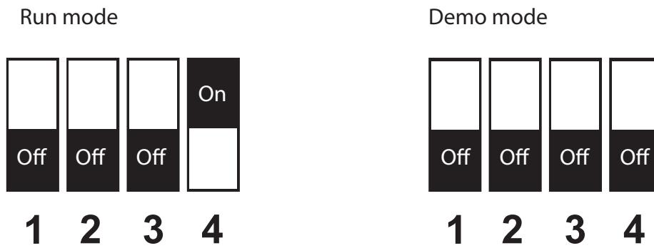
Figure 7: DIP switch run and demo modes
