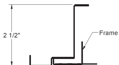
1" FILTER FRAME
