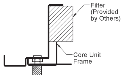
KNURLED KNOB FASTENER
