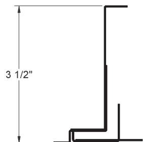
2" FILTER FRAME
