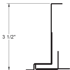
2" FILTER FRAME
