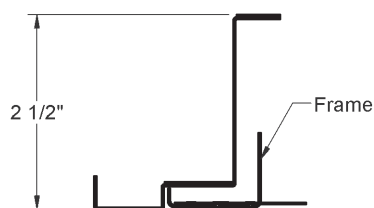
1" FILTER FRAME
