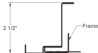
1" FILTER FRAME
