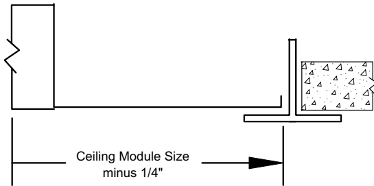
LT - Lay in T - Bar Detail
