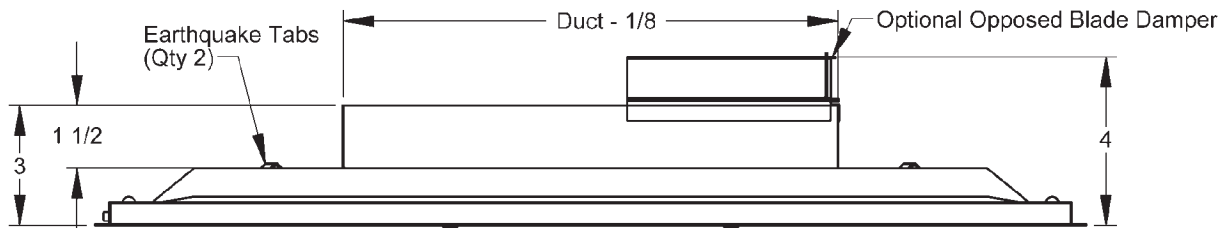
Side View/Damper Detail Square Neck
