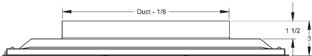
Side View Round Neck
