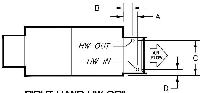
RIGHT HAND HW COIL (ARGT 3)
