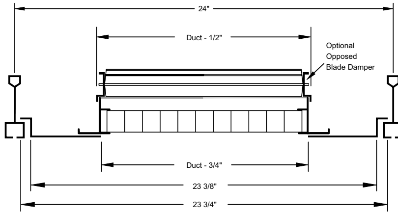
Side view/Damper Detail, NR (Narrow Regress) Frame *NR Frame is only available in 24"x24" module
