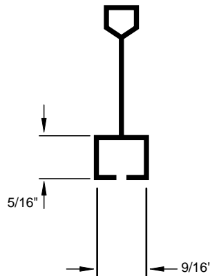
T - Bar Detail for NR Frame
